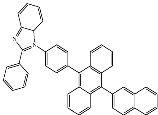
Compound H1
