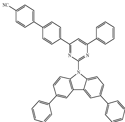
Compound H1
