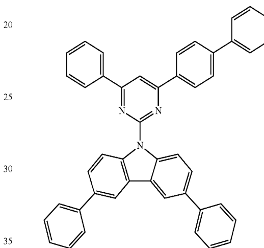
Compound F2
